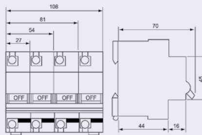
MCB4P-63DC
