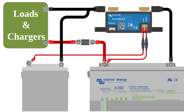
Battery monitor with auxiliary second battery monitoring.
